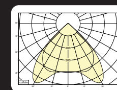
27113W.3340.90 Wide 33W 4000k 5500lm ηLB 100%
