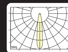
27113W.3340.30 Narrow 33W 4000k 5500lm ηLB 100%
