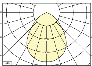
23008W.31D.RGBM 31w 2160lm ηLB 72%
